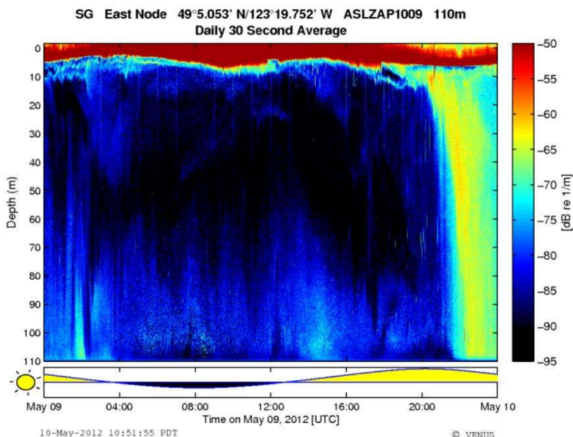
Figure 7. Cascade of suspended sediment as observed by a 200 kHz AWCP on the Ocean Networks Canada network on May 9, 2012 (ONC, 2018)
