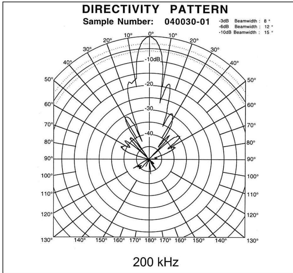
Figure 2. Example beam pattern for a 200 kHz transducer.
