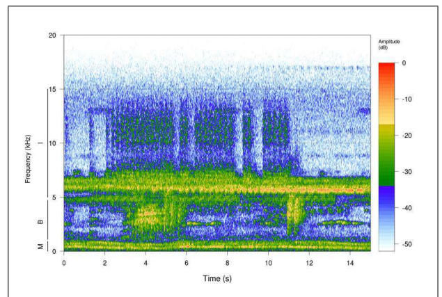
Figure 2. Sample of a community or soundscape recording. Spectrogram of a recording achieved at the Nouragues reserves in French Guiana on the 12nd of December 2010 at 6:30 am (point 04°05'18.99" N, 52°40'27.68" W). The recording include one mammal species (howler monkey, M) and several bird (B) and insect (I) species with lines indicating approximate respective frequency bands. Spectrogram specifications: 512 samples non-overlapping Hamming window with a 52 dB dynamic range. See [40] for details.
