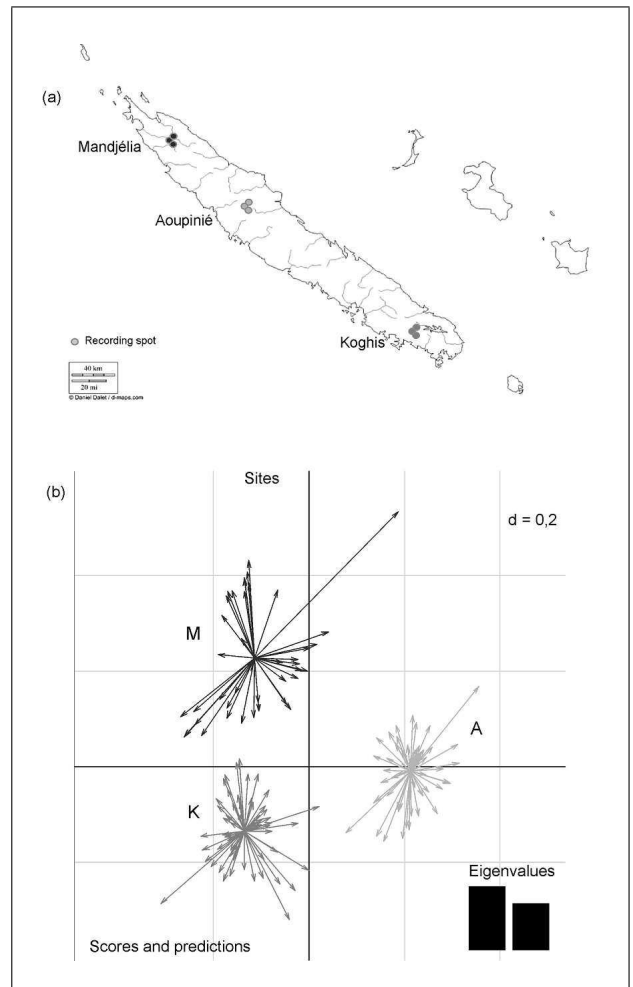
Figure 4. \beta acoustic diversity at a regional scale in New Caledonia. (a): The sound of three acoustic communities were sampled in three sites with three recording points at each site: Aoupinié (A), Koghis (K) and Mandjéla (M). (b): Results of Redundancy Analysis applied to the principal coordinates analysis of acoustic distances among all recordings, with a factor “Site” as an explanatory variable, revealing a clear acoustic difference between the three acoustic communities. The length of the arrows represents residuals: each arrow connects the position of a recording predicted by the site in which it was done (where the arrow starts) to its real position based on raw data (real acoustic composition where the arrow ends). Modified from [60].
